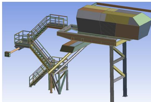
Figure 58: Retractable platform on ship Stresses on wheel & girder
