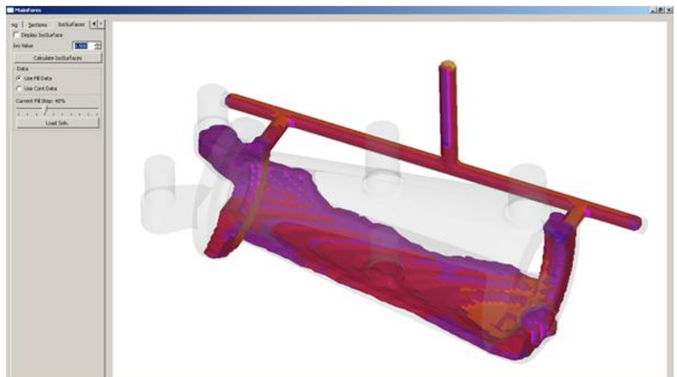
Figure 59: Visualization of hot spots in metal casting
